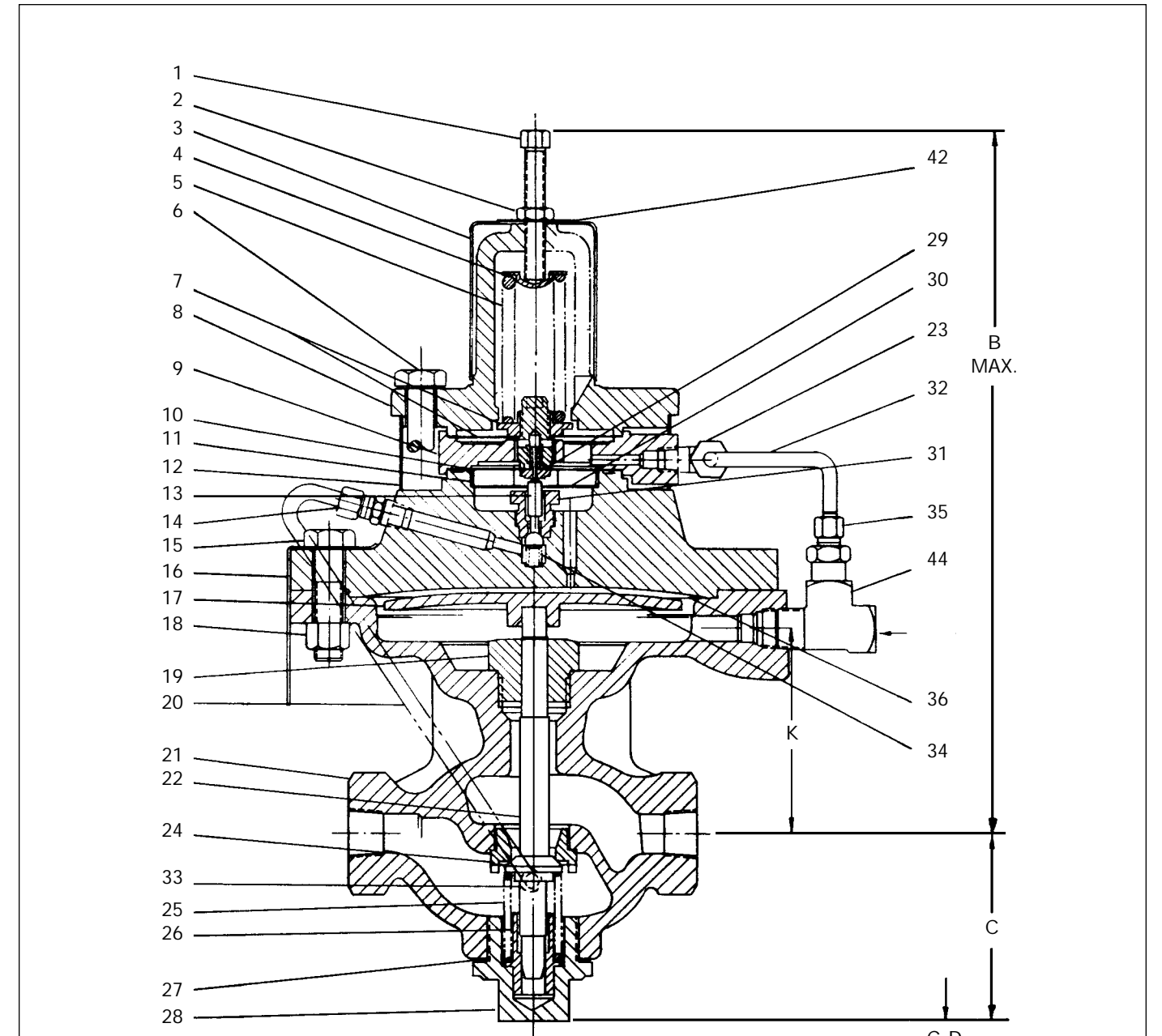
VIEW SHOWING 1/2" TO 2" SIZES WITH THREADED ENDS
